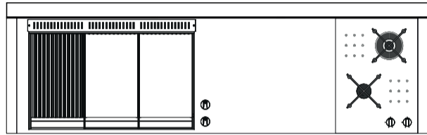
B.IN80GRILL. R/LL : Dimensioni piastra - Dimensions Plaque Plate's Dimensions - Platte Abmessungen: 26 + 26 + 26 cm
