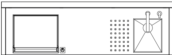
IN EL55 + lav / Dimensioni piastra - Dimensions Plaque Plate's Dimensions - Platte Abmessungen: 53 cm x 40 cm
