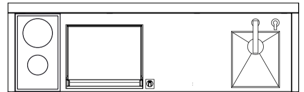
IN EL55 + INDU + LAV / Dimensioni piastra - Dimensions Plaque Plate's Dimensions - Platte Abmessungen: 53 cm x 40 cm
